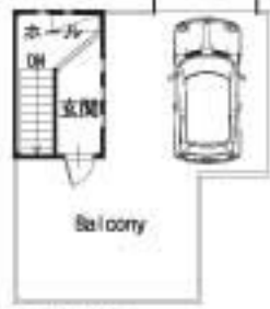
3F PLAN
